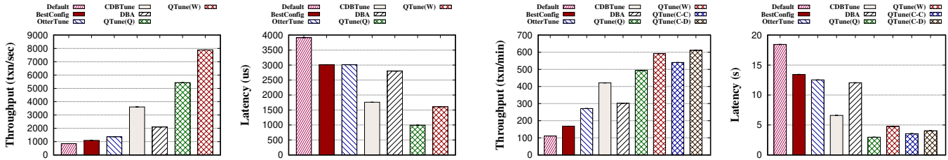
(a) JOB(RO) to Sysb.(RW) (b) JOB(RO) to Sysb.(RW) (c) TPC-H(RO) to JOB(RO) (d) TPC-H(RO) to JOB(RO)
