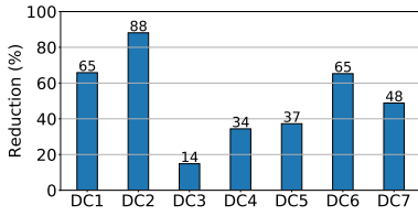
Figure 8: Cross-DC bandwidth reduction by Yugong
