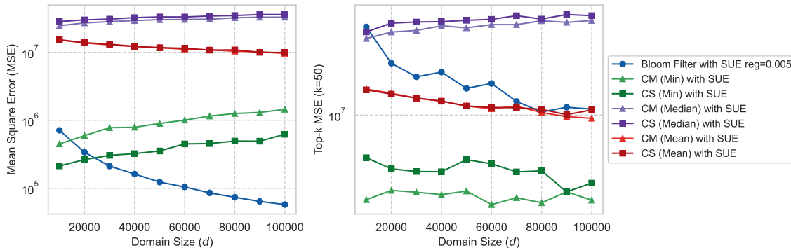
Figure 8: MSE (left) and k -MSE (right) comparison of Bloom-filter, Count-Min Sketch (CM) and Count-Sketch (CS) with Symmetric Unary Encoding (SUE). Fixing \epsilon = 3 , r = 16 , c = m = 128 on the Zipf distribution
