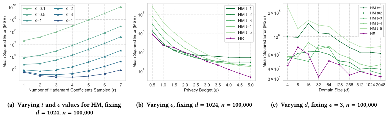
Figure 4: Hadamard Experiments
