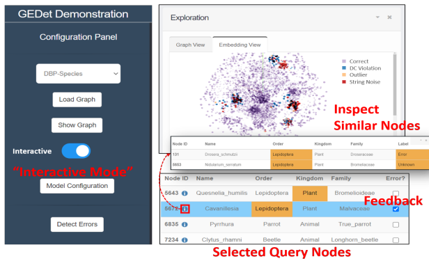
Figure 5: User Interface – Interactive Error Detection
