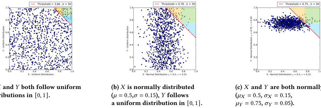
Figure 1: Top- k thresholds (score = 0.5X + 0.5Y ) based on the underlying distribution of values ( N=1000, k=50 ), X and Y are independent variables.
