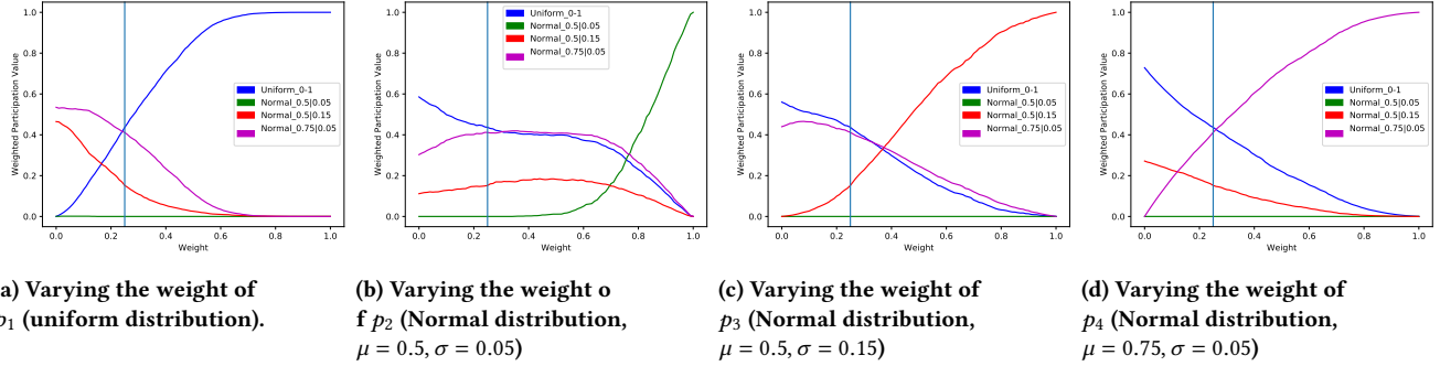
Figure 3: Weighted Participation of each parameter p as a function of the weight of each parameter P . For each plot, we vary the weight W_i of one parameter p_i , the other parameters weights are then computed as \frac{1-W_i}{3} .
