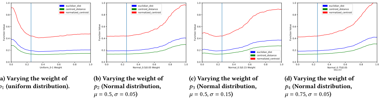
Figure 4: Distance Metrics: Euclidean Distance, Centroid Distance, and Normalized Centroid Distance (Diversity) as a function of the weight of each parameter P . For each plot, we vary the weight W_i of one parameter p_i , the other parameters weights are then computed as \frac{1-W_i}{3} .
