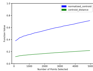
Figure 6: Centroid and Normalized Centroid Distance (Diversity) as a function of k
