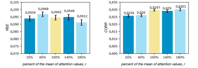
(c) Effect of adapted cut-off threshold r on RSE (Electricity) (d) Effect of adapted cut-off threshold r on CORR (Electricity)
