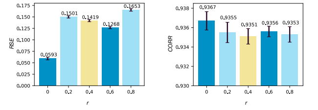
(e) Effect of fixed cut-off threshold r on RSE (Exchange Rate) (f) Effect of fixed cut-off threshold r on CORR (Exchange Rate)
