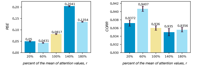
(g) Effect of adapted cut-off threshold r on RSE (Exchange Rate) (h) Effect of adapted cut-off threshold r on CORR (Exchange Rate)
