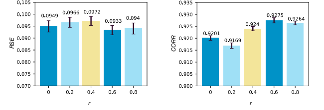
(a) Effect of fixed cut-off threshold r on RSE (Electricity) (b) Effect of fixed cut-off threshold r on CORR (Electricity)
