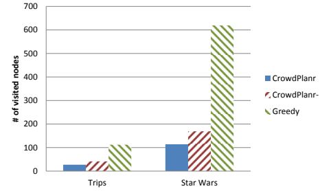
Figure 6: Real-world datasets
