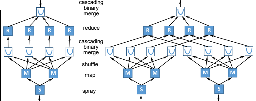
Figure 3: Two-stage streaming temporal map-reduce (one and two inputs).
