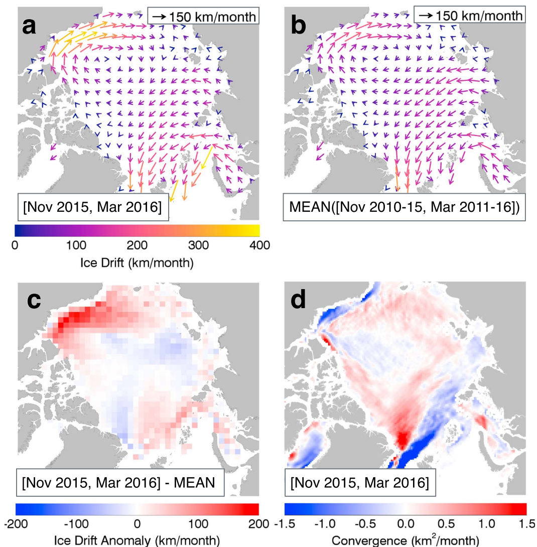
Figure 3. (a) CERSAT/IFREMER sea ice drift, averaged over November 2015–March 2016, and (b) winter ice drift averages for November 2010–March 2011 to November 2015–March 2016. (c) Ice drift magnitude anomaly of November 2015–March 2016. For better visualization in Figures 3a–3c, ice drift data are resampled on a 200 km grid. (d) Ice volume flux convergence of November 2015–March 2016. Positive values indicate convergence, while negative values indicate divergence.
