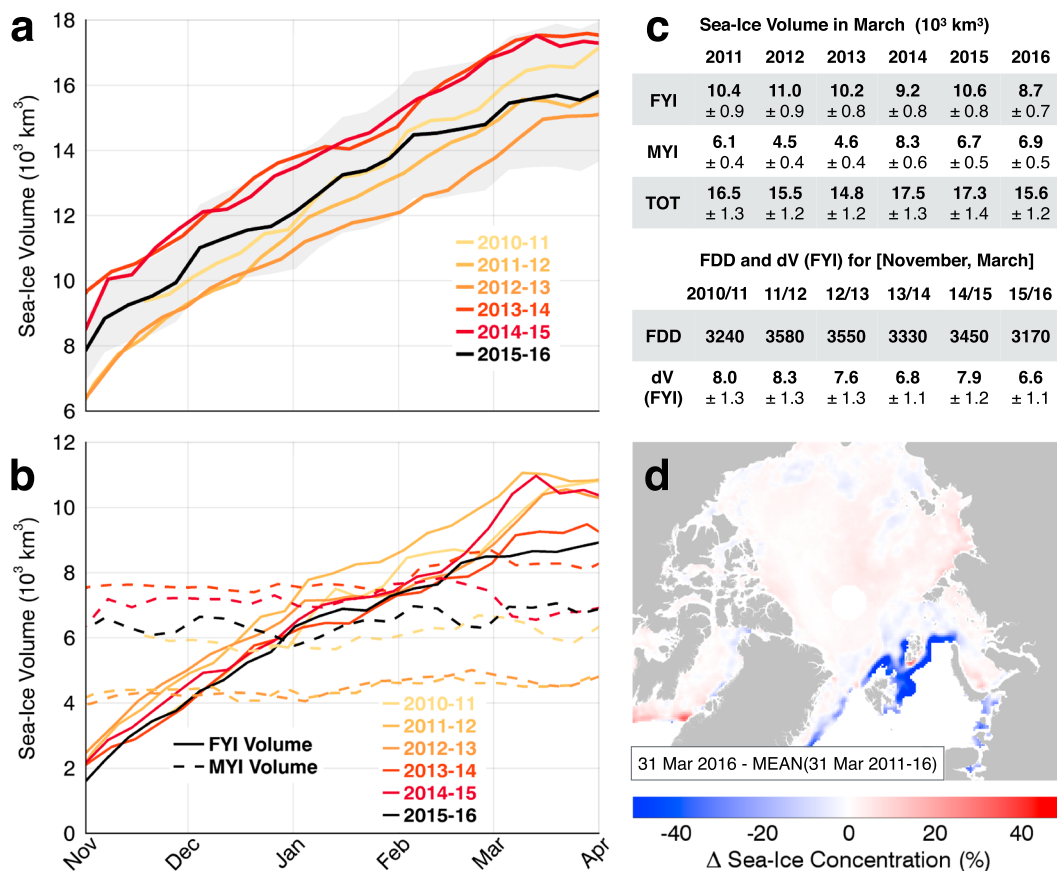
Figure 4. (a) Northern Hemisphere total sea ice volume for 2010–2011 to 2015–2016. Ice volume data stop end of March because ice thickness cannot be retrieved during melting. The grey shadowed area represents the ice volume uncertainty for 2015–2016. (b) First- and multiyear ice (FYI/MYI) volume contributions to the total volume. (c) March ice volume averages and corresponding uncertainties from 2011–2016, as well as spatially averaged FDD over FYI, cumulated from November to March, and corresponding sea ice volume gain (dV). (d) Sea ice concentration anomaly for the 31st of March 2016 with respect to the average of the 6 year record.
