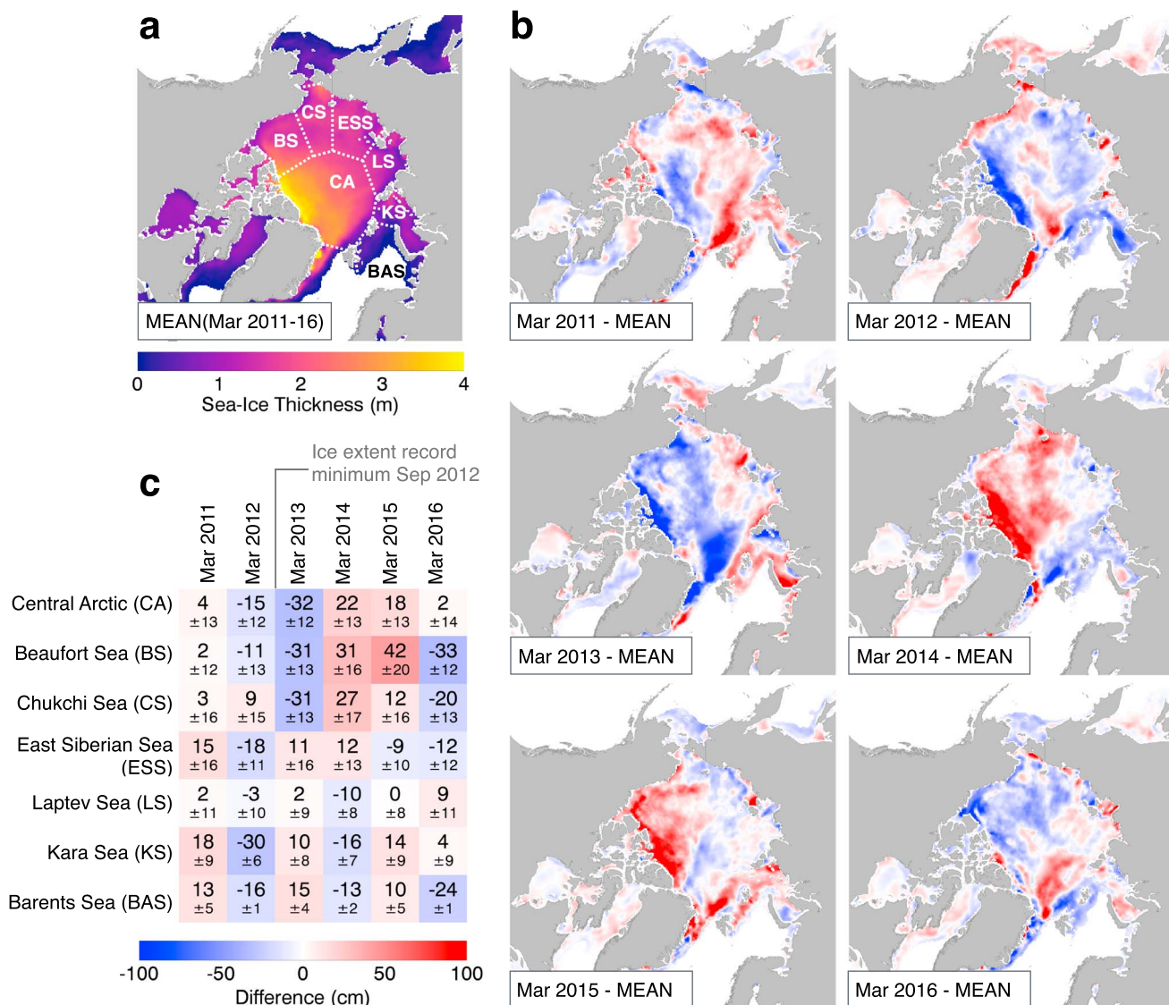
Figure 2. Merged CryoSat-2/SMOS sea ice thickness anomaly for a mean of 3 weeks in March according to the March thickness averaged over 2011–2016: (a) March average over 2011–2016, subdivided into maritime boundaries provided by NSIDC via MAISIE. (b) Yearly March anomalies. (c) Mean anomalies and uncertainties of each year according to the March 2011–2016 mean with respect to the marine domains defined in Figure 2a.
