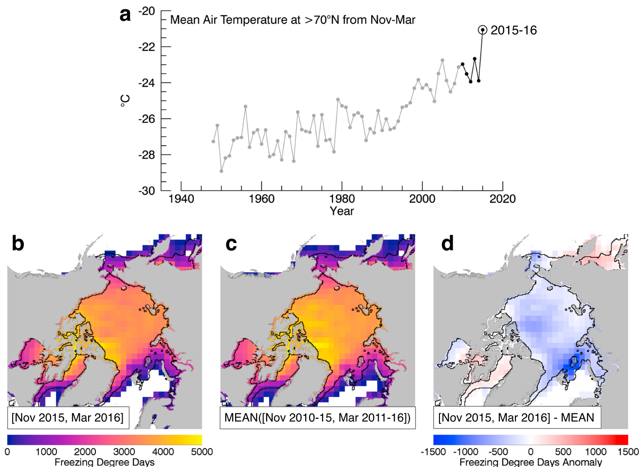
Figure 1. (a) Mean air temperatures above 70°N during November 1948–March 2016, derived from the National Centers for Environmental Prediction (NCEP) monthly reanalysis air temperature, 2 m above surface. (b) Mean Cumulative freezing degree days (FDD) calculated from NCEP air temperature data for November 2015–March 2016. (c) Winter average of FDD for November 2010–March 2011 to November 2015–March 2016. (d) Winter 2015–2016 compared to the winter mean. The black line highlights the mean ice edge during March 2016.
