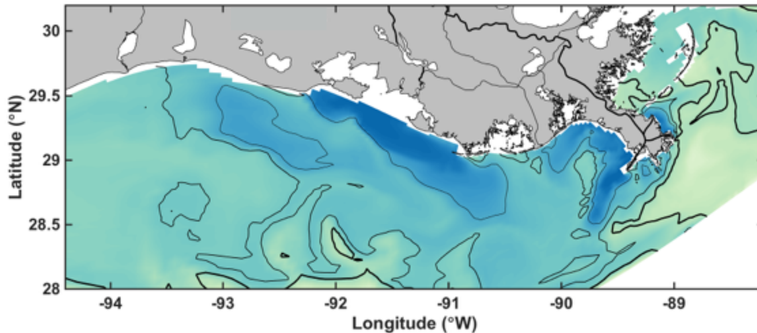
Mid-summer surface salinity (future)
