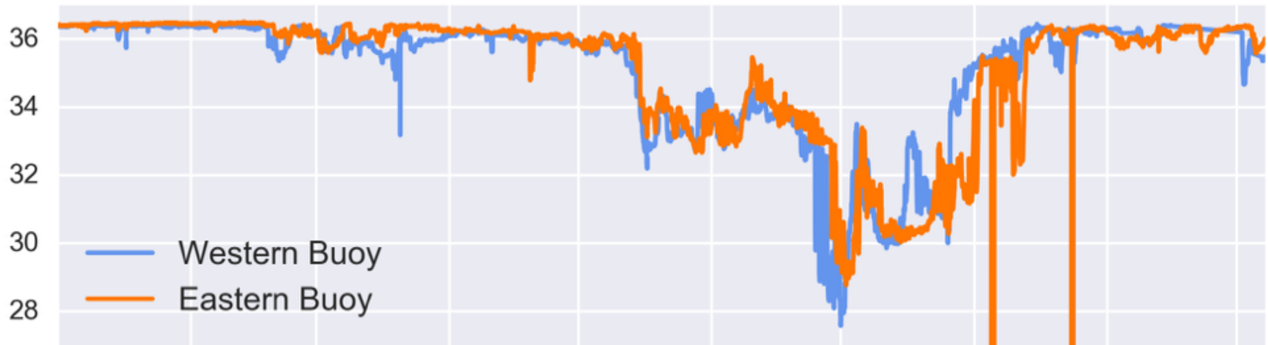
Surface salinity
