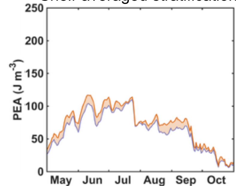
Shelf-averaged stratification
