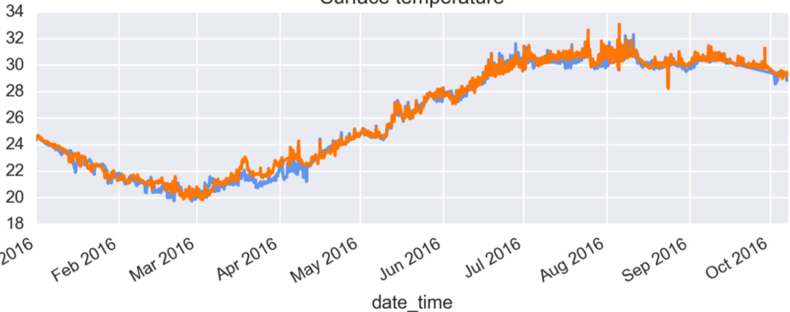
Surface temperature
