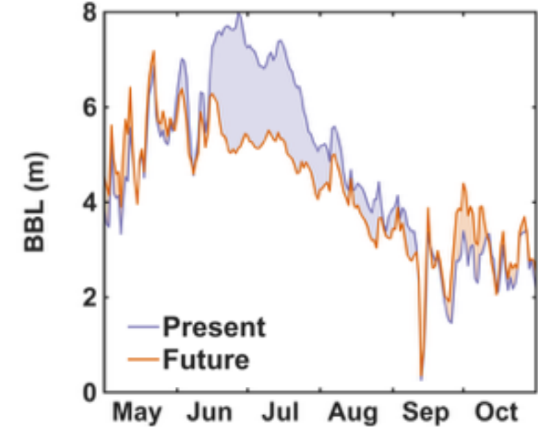
Shelf-averaged BBL thickness
