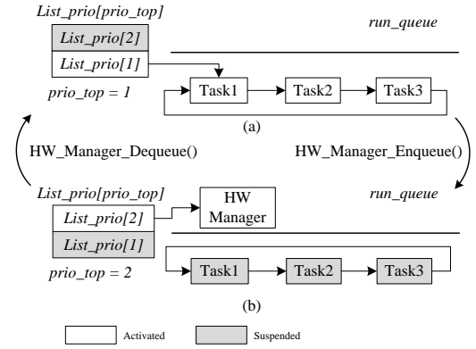
Figure 3: Microkernel Scheduling Mechanism. (a) prio\_top=1 ; (b) prio\_top=2
