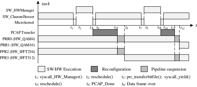
Figure 5: Gantt Chart of the Tasks' Execution
