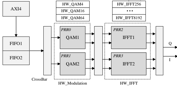
Figure 4: Use-Case Implementation
