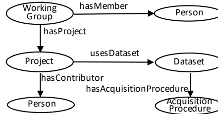
Figure 1: Core classes of the collaboration ontology.
