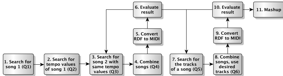
Fig. 1. The mashup creation framework
