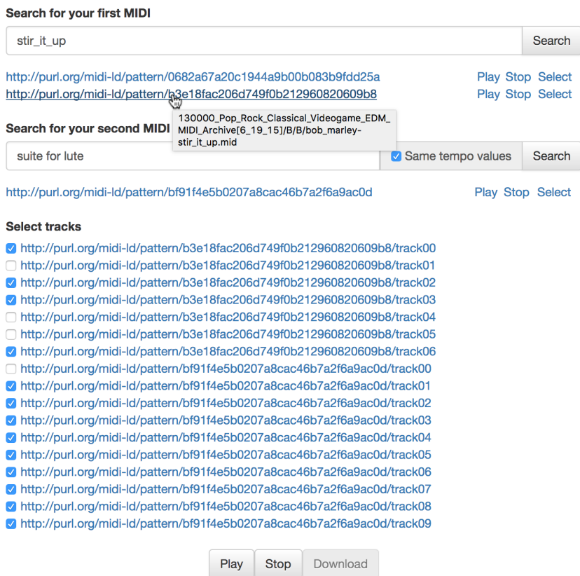
Fig. 3. A screenshot of the SPARQL-DJ tool
