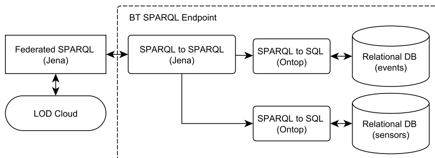
Fig. 1. BT Data Hub Architecture.
