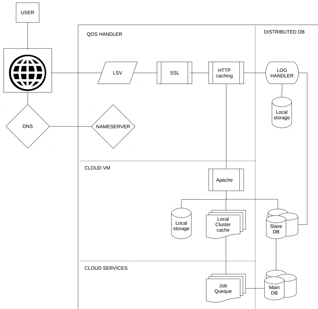
Figure 2: Schematics of the services involved in developed system and the respective dependencies.
