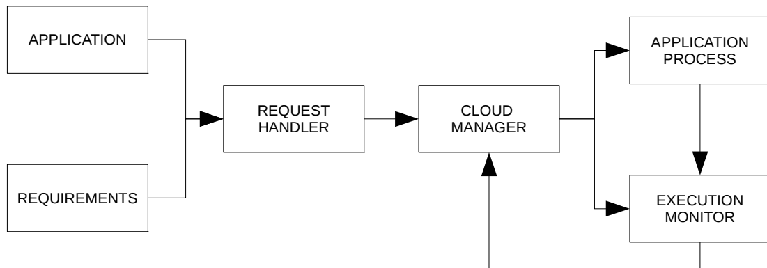
Figure 4: Schematics of the Cloud Administration Service (CAS).
