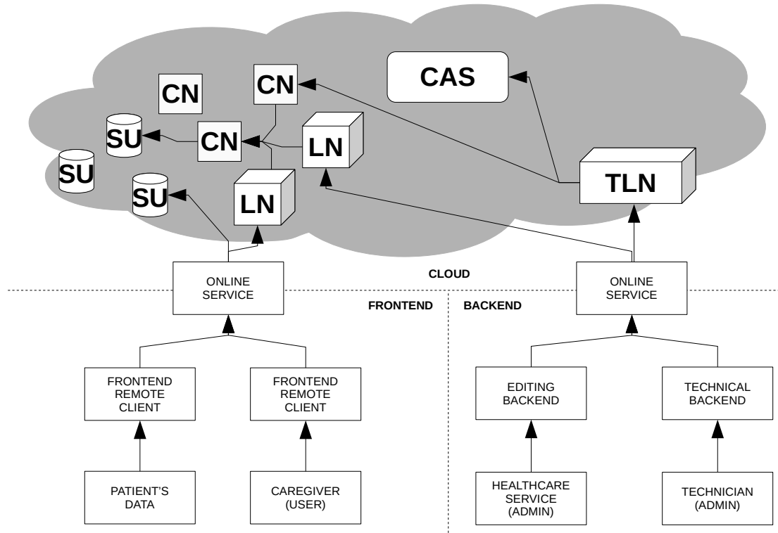
Figure 1: A general schema of the system developed in this work. Clockwise: a representation of the cloud and its resources, the administrative and test design backend, and, finally, the users' frontend.
