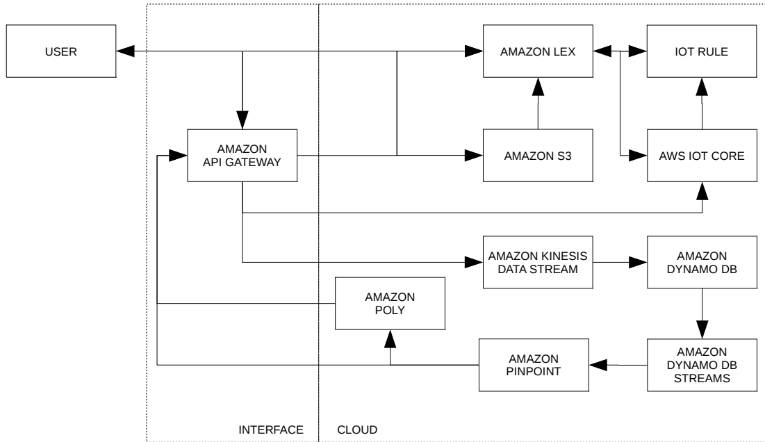
Figure 3: The adopted Amazon Web Services (AWS) configuration and the relative data flow among the different component and services within the cloud environment
