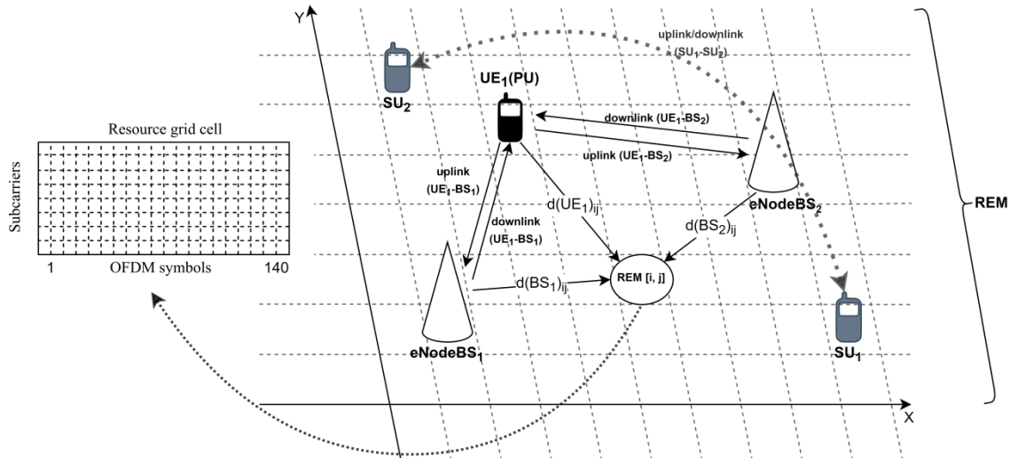
Figure 1: A cognitive system simulation model representation based on LTE
