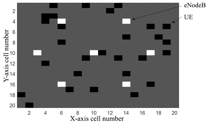
Figure 5: An example of the eNodeB and UE objects initial location on the map in the model
