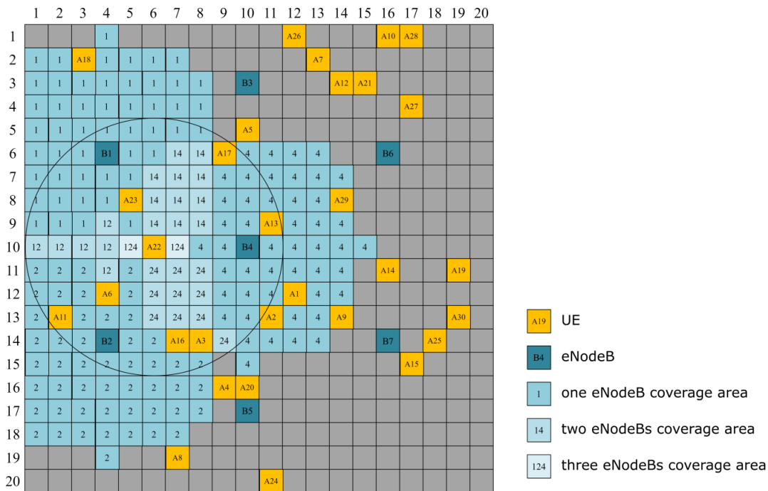
Figure 7: Schematic location of eNodeB and UE objects on the REM and radio visibility area at the point (6, 10)
