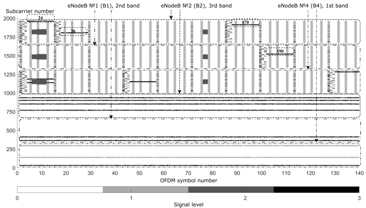
Figure 8: Radio environment between the UE and the workstation at the point (6, 10)
