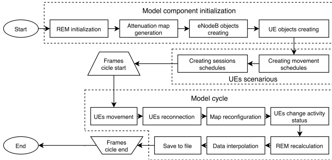
Figure 2: REM generation algorithm
