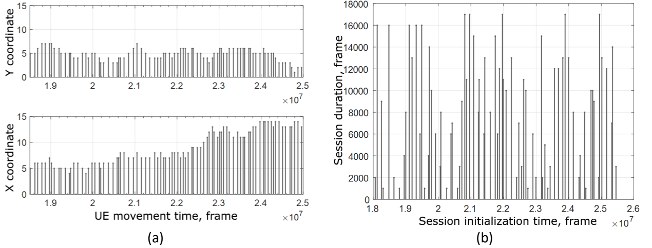
Figure 3: UE scenarios: position change according to the "Courier" scenario (a), sequence of sessions according to the "User" scenario (b)
