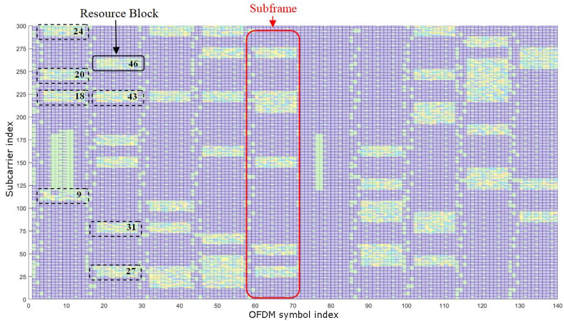
Figure 4: eNodeB downlink resource grid
