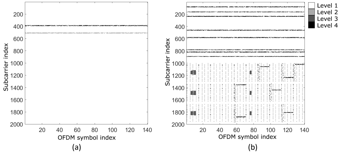
Figure 6: Network traffic at the edge of the map (a); near the station (b) – 1 – no signal (below -120 dBm); 2 - weak level, UE shutdown (up to -83 dBm); 3 – medium level (up to -20 dBm); 4 - strong level (above -20 dBm).
