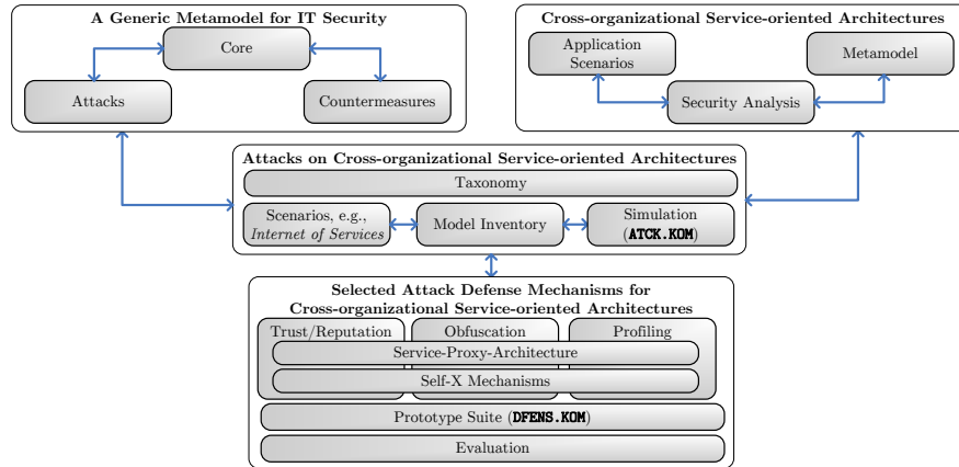
Figure 1. Research structure and approach
