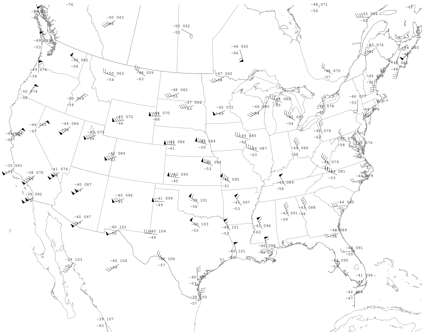
250 mb Observations Valid 240920/0000 UTC College of DuPage NEXLAB
