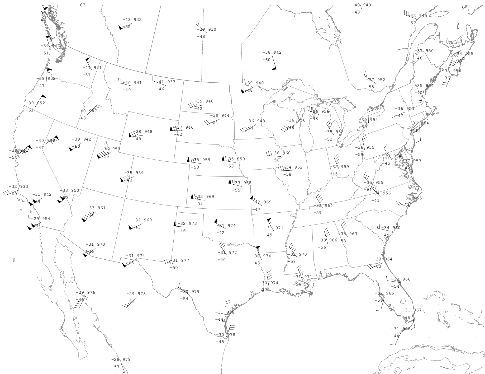
300 mb Observations Valid 240920/0000 UTC College of DuPage NEXLAB
