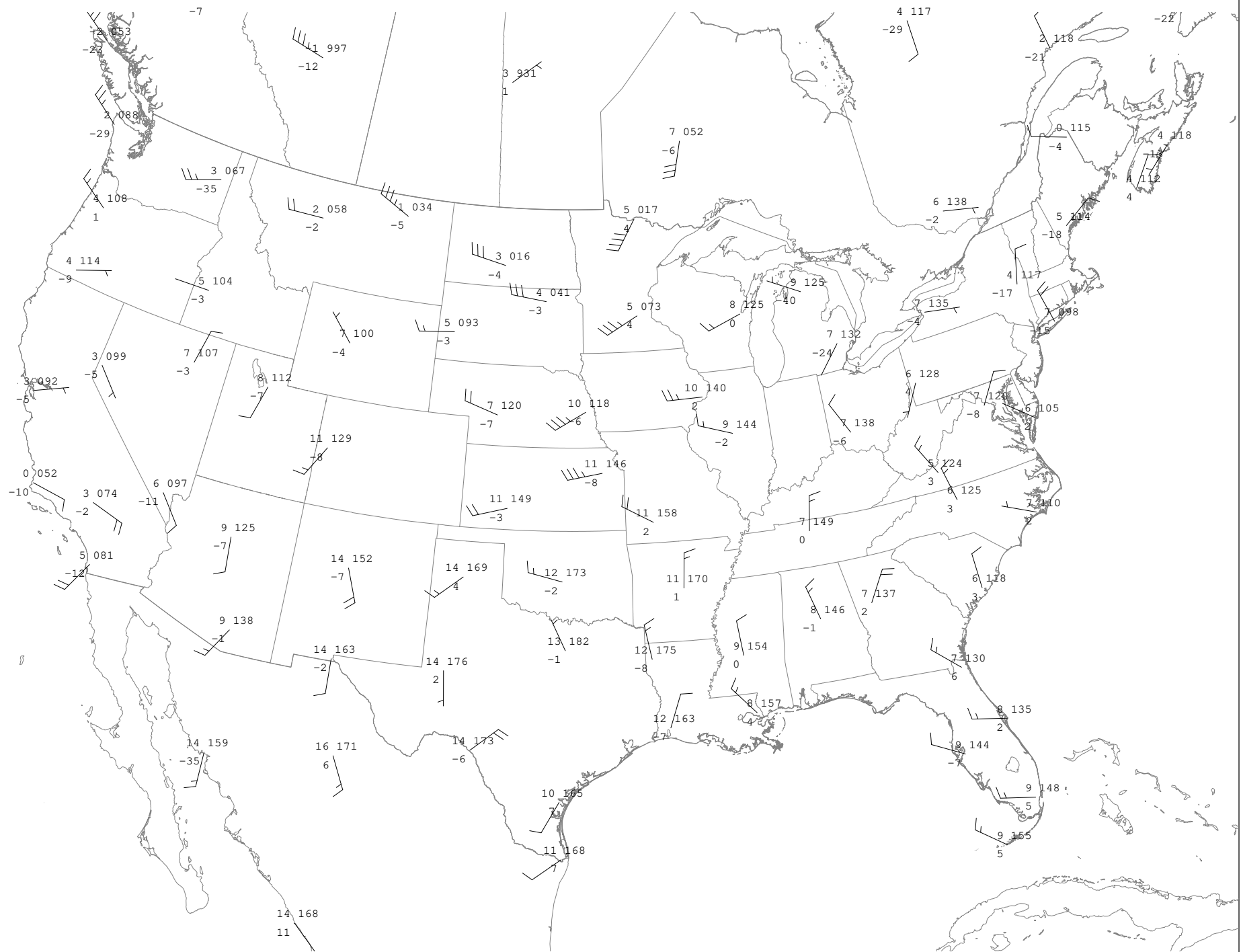
700 mb Observations Valid 240920/0000 UTC College of DuPage NEXLAB
