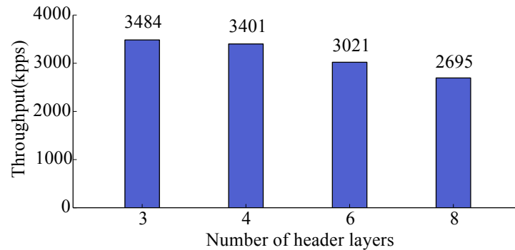
Figure 3.6: Single parser performance with different packet headers.
