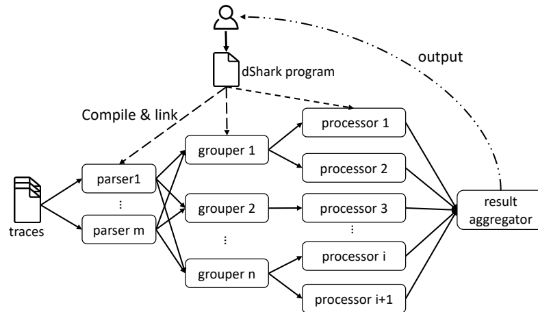
Figure 3.2: DSHARK architecture.
