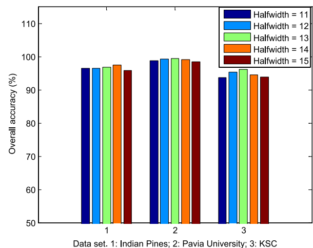
Fig. 19. Influence of spatial size on the (left) Indian Pine, (middle) University of Pavia, and (right) KSC data sets. Best view in color.
