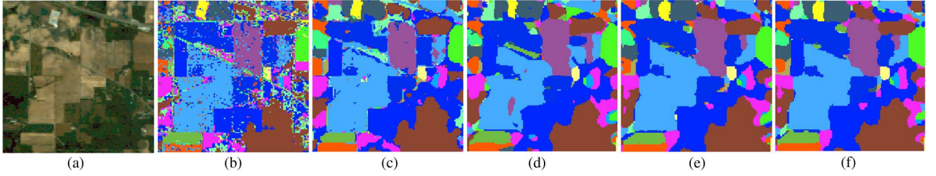
Fig. 20. Indian Pines. (a) False color image. (b)–(f) Classification maps for different classifiers: (b) 1D-SVM, (c) 3D-EMP-SVM, (d) 3D-CNN, (e) 3D-CNN with Method A, and (f) 3D-CNN with Method B.
