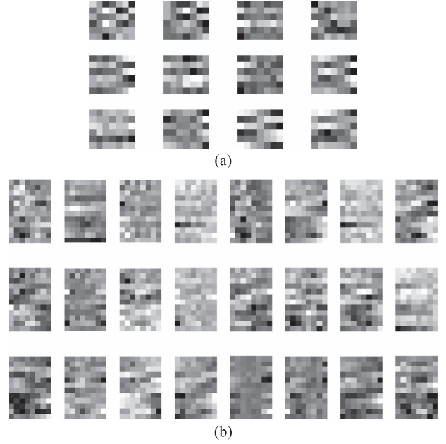
Fig. 12. Weights of the second and third convolutional layers on the University of Pavia data set. In the first column of the image, there are 12 filters, and each tiny image contains 42 ( 6 \times 7 ) weights of a convolutional kernel. The second one shows 24 filters and 96 ( 12 \times 8 ) weights in a tiny image. (a) Learned weights of the second convolutional layer. (b) Learned weights of the third convolutional layer.
