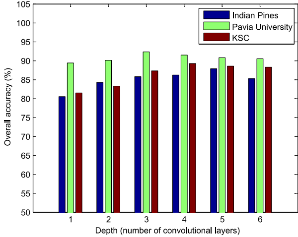
Fig. 10. Spectral information-based classification results of different depths using CNN.
