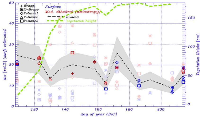
Fig. 15. Estimated mean soil moisture over the rape field 101 in time inverted from the (blue) surface and (red) dihedal scattering components as obtained from the different decomposition approaches. The ground-estimated soil moisture is indicated by the black dashed line, and the \pm 30\% variation region is indicated in gray region. The vegetation height is given by the green dashed line.
