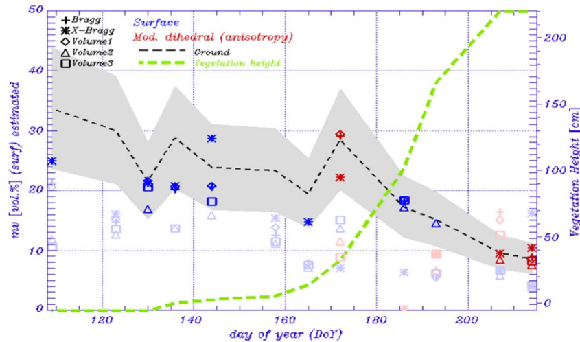
Fig. 17. Estimated mean soil moisture over the corn field 222 in time inverted from the (blue) surface and (red) dihedal scattering components as obtained from the different decomposition approaches. The ground-estimated soil moisture is indicated by the black dashed line, and the \pm 30\% variation region is indicated in gray region. The vegetation height is given by the green dashed line.
