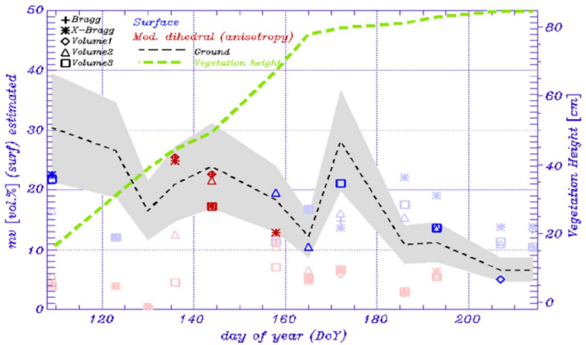
Fig. 16. Estimated mean soil moisture over the wheat field 230 in time inverted from the (blue) surface and (red) dihedal scattering components as obtained from the different decomposition approaches. The ground-estimated soil moisture is indicated by the black dashed line, and the \pm 30\% variation region is indicated in gray region. The vegetation height is given by the green dashed line.
