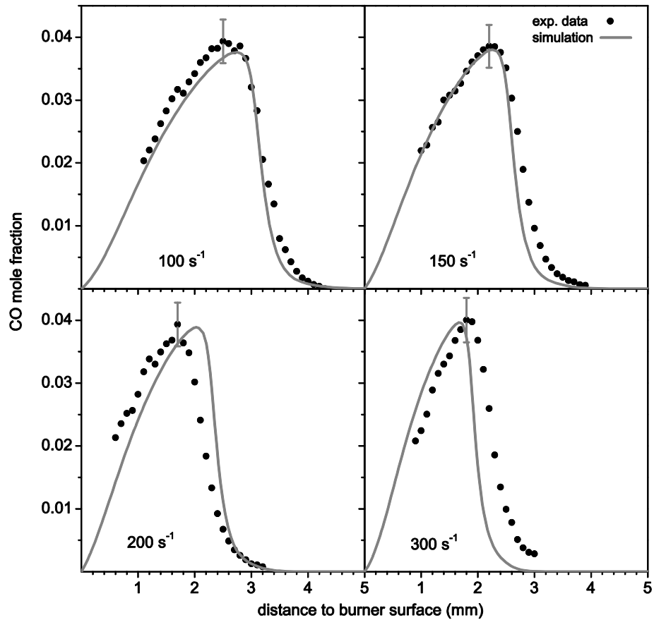
Figure 7 Comparison of the measured and simulated CO concentrations profiles for flames with strain rates between 100 and 300 \text{s}^{-1} . The experimental data (dots) are reproduced very well from the model based simulation (line). The shape, position and absolute values of the measured profiles agree excellent over a broad range with the simulated data.
