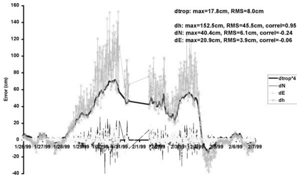
Figure 8. Effect of EGNOS model zenith tropospheric delay errors on position quality for Lerwick for a 5 degree elevation cut-off, all observations equally weighted.
