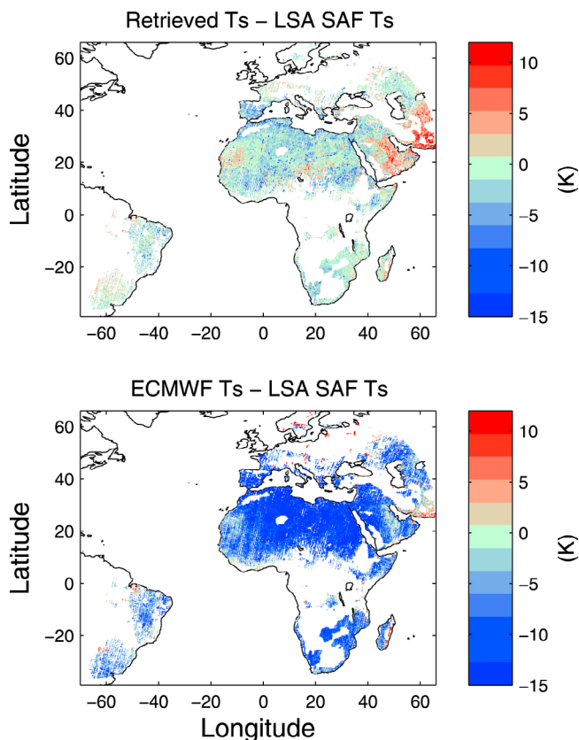
Figure 12. Retrieved (top) T_s minus LSA SAF T_s and (bottom) ECMWF T_s minus LSA SAF T_s . All data from the first week of January, April, July, and October are gathered on the map.
