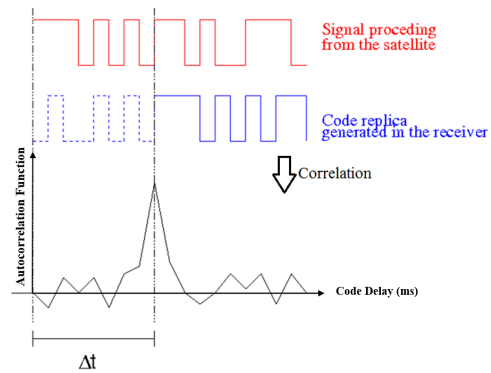
Fig. 8. Principle of GNSS code delay tracking [72]
