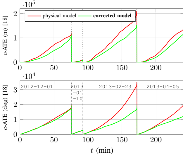
Fig. 4. Translation (above) and rotation (bottom) cumulative Absolute Trajectory Error ( c -ATE) as function of time for physical and corrected models for four sequences of Segway dataset [18]. Errors are set to zero when starting a new sequence. The proposed corrected model accumulates lower error residual than the physical model.
