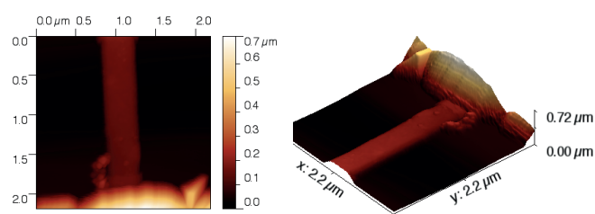
Fig. 4. AFM image of the active area of a fabricated SiNW-FET.
