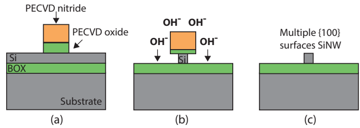
Fig. 1. Process-flow for the fabrication of silicon nanowires. (a) Silicon oxide and nitride hard mask patterning; (b) Silicon etching with KOH; (c) Nitride and Oxide removal ( \text{H}_3\text{PO}_4/\text{BHF} ).
