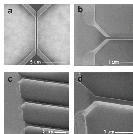
Fig. 3. SEM images of the fabricated SiNW-FETs.
