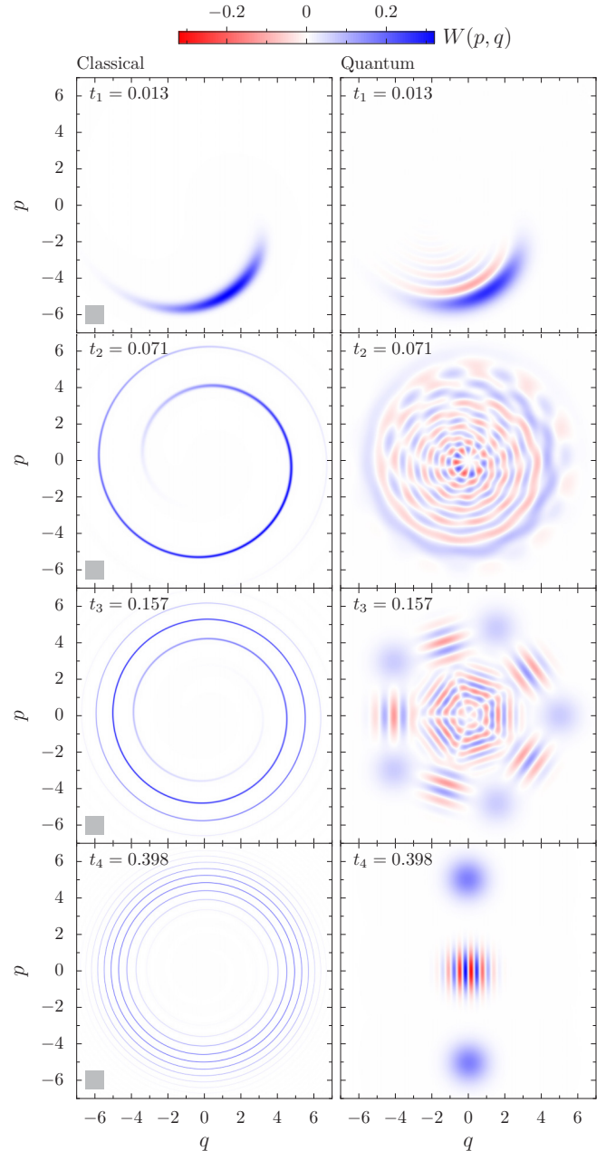
FIG. 1. The classical and quantum Wigner functions of a coherent state initially centered at the phase-space point (q, p) = (5, 0) are displayed for four different times, with the largest one exceeding 6T_E , the Ehrenfest time for this case being given by (6) as T_E \approx 0.063 . The times t_3 = T_{\text{rev}}/5 and t_4 = T_{\text{rev}}/2 correspond to fractional revivals, where T_{\text{rev}} is given by (5). The gray squares in the classical plots represent regions of area \hbar .
