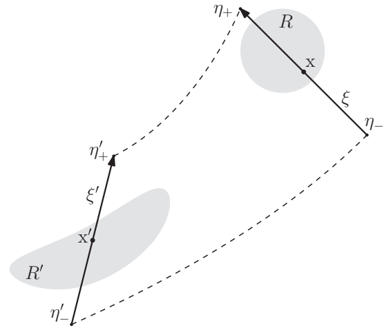
FIG. 2. A final chord \xi' , with center x' , is evolved backwards to form an initial chord \xi(\xi', x', t) , centered at x(\xi', x', t) . By considering the endpoints of \xi' and \xi , such evolution is described by the circuit \eta'_- \mapsto \eta_- \mapsto \eta_+ \mapsto \eta'_+ . The first and last propagations are performed along classical trajectories (dashed lines), while the middle one is a reflection around x , given by \eta_+ = 2x - \eta_- . The shaded areas R and R' represent the Wigner function at initial and final times, respectively.
