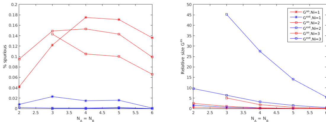
Figure 4: Performance of the extended asymptotic graph method for asynchronous networks (darker curves, G_*^{ext} ) and comparison with original method (lighter curves, G_*^a ), for randomly generated modules, and interconnected networks with p_A = 1, 2, 3 . Left: the percentage of failure (i.e., the generation of spurious). Right: the sizes of both asymptotic graphs relative to the size of the full network G_*^I .
