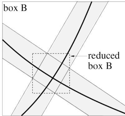
Figure 8: Linearization by intervals of a 2D system within a box B . The two involved curves are enclosed in two thick lines represented by the two gray-shaded bands. The solution of this 2D system is represented by the reduced box drawn in dashed lines.
