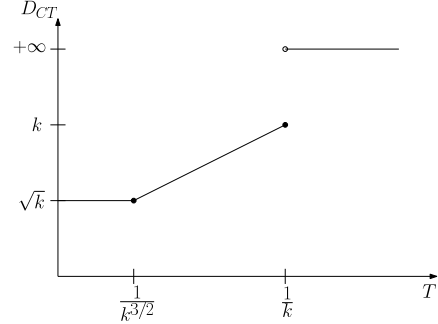
Fig. 2. Complete team policy: Delay versus throughput.
