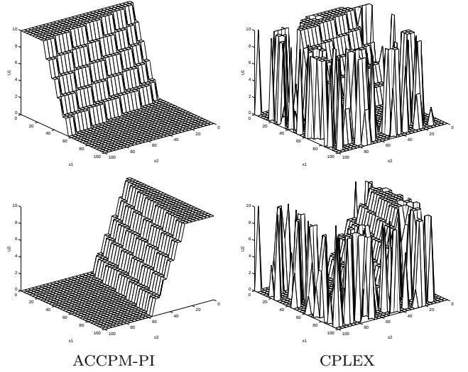
Figure 4: Optimal policy.
