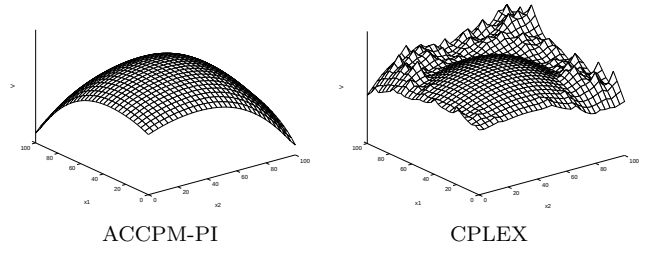
Figure 3: Value function.
