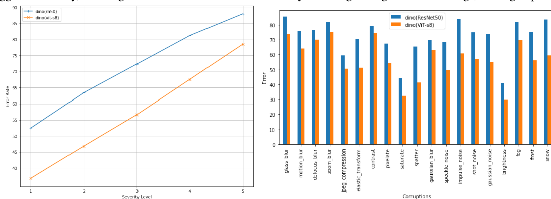
Figure 4. Comparison between different backbones, ResNet50 and ViT-s8 for DINO SSL method over ImageNet-C [25] corruptions. Severity levels (left), corruptions (right).
