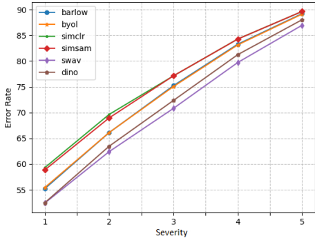
Figure 1. Error rates vs. severity levels across ImageNet-C [25] corruptions.
