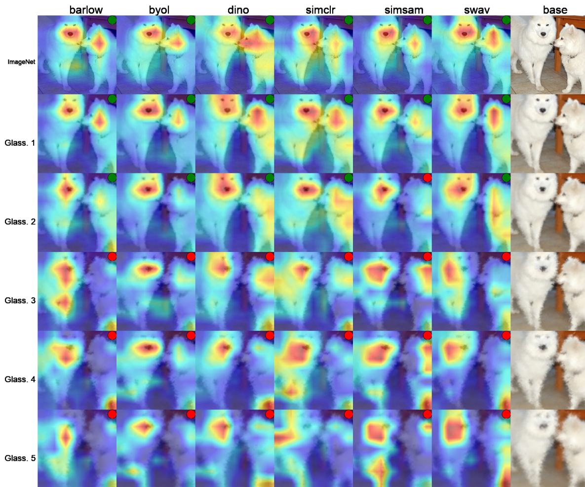
Figure 3. Glass blur on dogs; markers in the images show correct (green) and incorrect (red) classifications. In ImageNet, with many dog breed classes, misclassification doesn't necessarily indicate a bad model if the representation is adequate. In the twin dog example, with low blur severity, both dogs have good activations for all models, suggesting good representations. However, at high blur severity, the model struggles to classify, resulting in distorted activations and difficulty in distinguishing between the dogs, leading to poor results.
