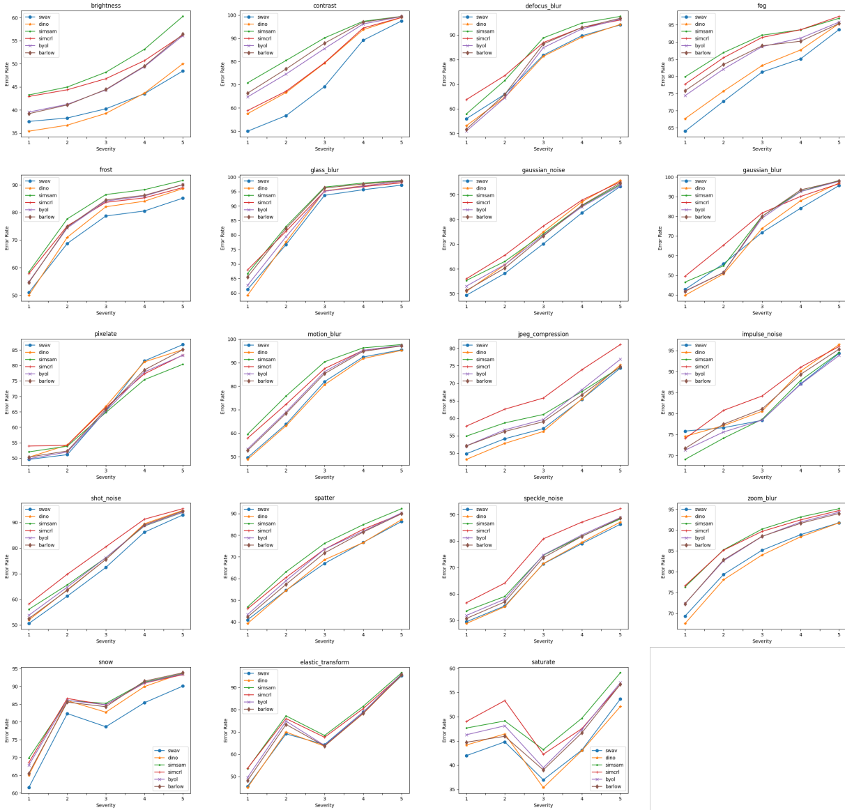
Figure 2. Model performance against specific corruptions by severity. For corruptions, namely, snow, saturate, and elastic (last row), SSL models perform poorly at severity level 2 than at severity level 3.
