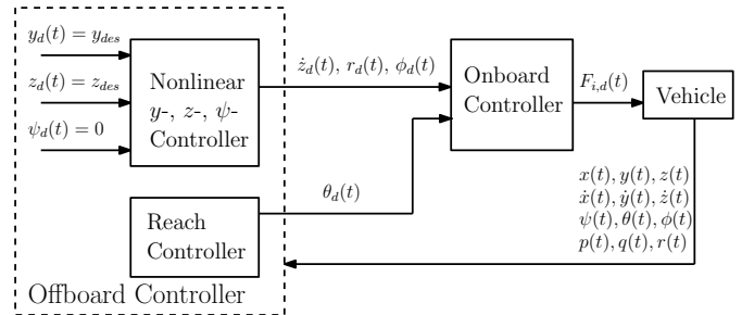
Fig. 3. The control architecture.
