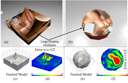
Fig. 3: The cuboid and icosphere are subjected to large deformation ((a) & (b)) with large, floating objects flying across the scene (as occlusion). The tracking output is shown in (c) and (e) while \mathbf{E}_{\text{depth}} is shown on the surface of S in (d) and (f)
