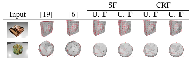
Fig. 2: Comparison between GT and tracking output for the two synthetic sequences cube and icosphere . The red edges and vertices shows the object model from the GT, the black ones are from the tracking output.
