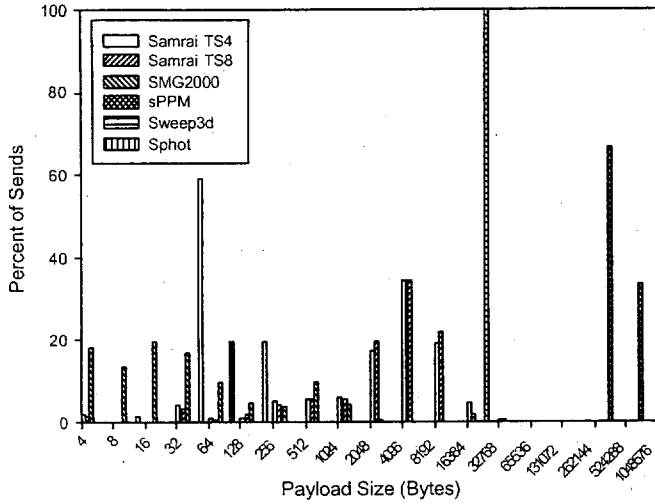
Figure 1: Payload size distribution for P2P messages (64 tasks).
