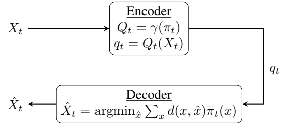
Fig. 1. Block diagram for our zero-delay coding system: X_t is the source sample, q_t is the encoded symbol transmitted through the noiseless channel, and \hat{X}_t is the reconstructed source sample.
