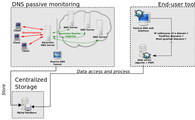
Fig. 4: DNSSM Architecture
