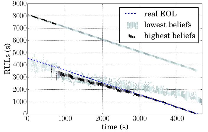
Fig. 8. Battery parasitic load fault scenario - RUL estimates with (40, 80, 1500)_\Delta and (1, 5, 100)_\Pi .
