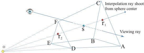
Figure 4: Barycentric interpolation of the scalar value within a triangular frustum. We first interpolate the scalar values at the points \mathbf{r}_1 and \mathbf{r}_2 on the top and bottom triangles, respectively, and then use linear interpolation to compute the scalar value at the point \mathbf{s} on the line segment \mathbf{r}_1\mathbf{r}_2 .
