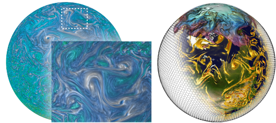
Figure 7: Ray-casting with lighting effects using our analytic ray integration and gradient estimation on the high resolution data set. The left images show the vorticity variable and the close-up view of a selected region. The right image shows the combination of grid illustration, volume rendering of vorticity (yellow tubes) and temperature (north cap). Our approach can succinctly reveal great details from large data with enhanced depth and shape cues.
