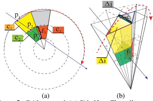
Figure 3: Grid traversal. (a) Side View. The yellow, green, and red frusta are constructed on the fly with marching the ray through the grid. The intersection of the ray and a temporary frustum is used to identify the next neighboring triangle on the spherical surface. (b) Perspective View. The red dashed curve is the projection of the ray on the spherical surface. The triangles \Delta_i and \Delta_j are identified based on the surface connectivity information, and are used to construct the corresponding frustum at the different layers.
