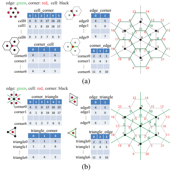
Figure 2: (a): The cell_corner , corner_cell , corner_edge , and edge_corner tables used to represent a 2D Voronoi grid of climate simulations. (b): The representation of dual triangular mesh of (a). We note that the names of tables and table entries are modified for an illustration purpose in (b), and they are not changed in the real implementation. Thus, from (a) to (b), the content of the four tables keeps intact, which implies that no explicit grid transformation is required.
