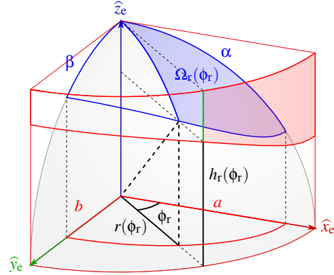
Figure 5: Illustration of our polar mapping. Projected perpendicularly to its axis \hat{z}_e onto the \hat{x}_e\hat{y}_e plane, the spherical ellipse forms a planar ellipse with semi-axes a = \sin \alpha and b = \sin \beta . We use the Pythagorean theorem to express the altitude h_r(\varphi_r) of the cylindrical projection of the spherical ellipse’s curve in terms of a , b , and \varphi_r .
