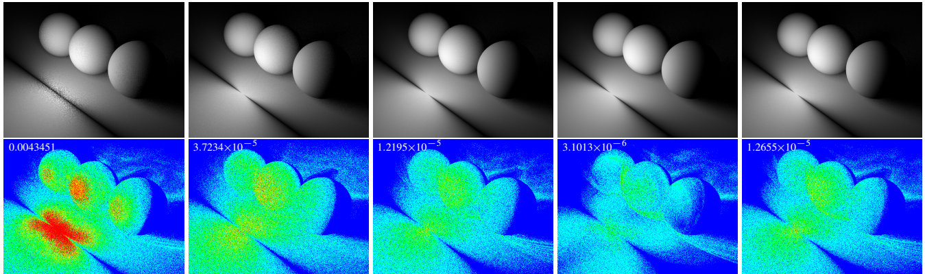
(a) Area sampling [SC97] (b) Gamito [Gam16] (c) Our parallel mapping (d) Our radial mapping (e) Our ld-radial mapping
