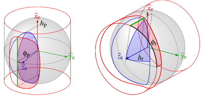
Figure 4: Illustration of our parallel (left) and radial (right) maps. Given a canonical sample (\varepsilon_1, \varepsilon_2) \in [0, 1]^2 , we first find the azimuth angle \phi_p , respectively \phi_r , that cuts a region on the cylindrical ellipse with area \varepsilon_1 \Omega_D (in red, determined by the green line segment). A sample point on the cylinder is then obtained by linearly interpolating the green segment endpoints using \varepsilon_2 . For the parallel map, the endpoint cylindrical coordinates are (\phi_p, -h_p) and (\phi_p, h_p) , with \phi_p \in [-\beta, \beta] . For the radial map, these coordinates are (\phi_r, h_r) and (\phi_r, 1) , with \phi_r \in [0, 2\pi] (we use \phi_r \in [0, \pi/2] in each quadrant).
