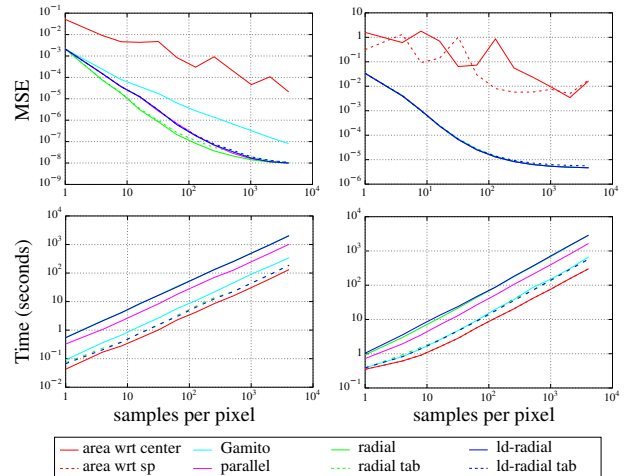
Figure 6: Error (top) and cost (bottom) for the results shown in Figure 7 (left) and Figure 8 (right), w.r.t. sample count.
