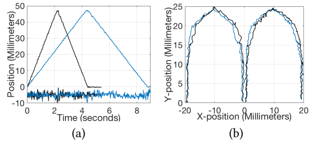
Figure 4: (a) Measured position and noise (amplified and offset) of the marble in slow (blue) and fast (black) motion mode. (b) Example of clockwise (black) and counterclockwise (blue) motion in both fast (left) and slow (right) mode.
