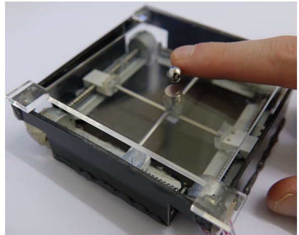
Figure 3: The prototype with its internal mechanism is shown. In our experiments, it was flipped and fixed upside down with the marble below the device.
