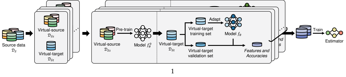
Fig. 6. An illustration of the training process of the performance estimator. We generate training data via simulation. The whole process runs on the developer side.
