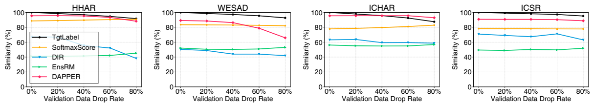
Fig. 9. Result with imbalanced target validation data.
