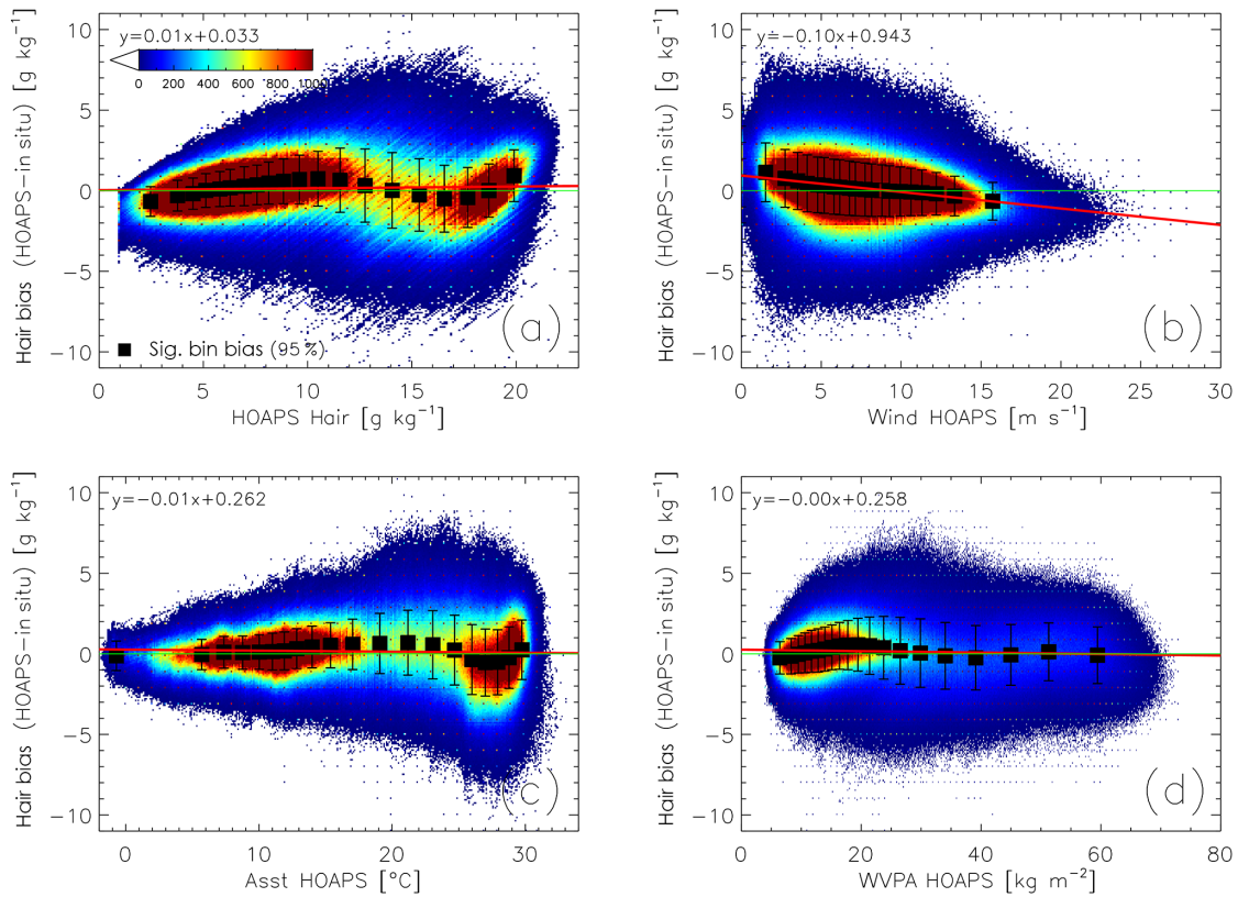
Figure 2. Scatter density plots of q_a bias (HOAPS 3.3 minus in situ, \text{g kg}^{-1} ) as a function of (a) q_a (“Hair”), (b) U (“Wind”), (c) SST (“Asst”), and (d) vertically integrated water vapour (“WVPA”), based on global double collocations between 2001 and 2008. The black squares and error bars represent bin-averaged systematic uncertainties (significant at the 95 % level) and their SDs, whereby each bin contains 5 % of all double collocated matchups. Note that the bars include random uncertainty contributions from the satellite retrieval, the collocation procedure, and the in situ measurement uncertainty. Panel (a) is a revised version of Fig. 3 published in Kinzel et al. (2016).
