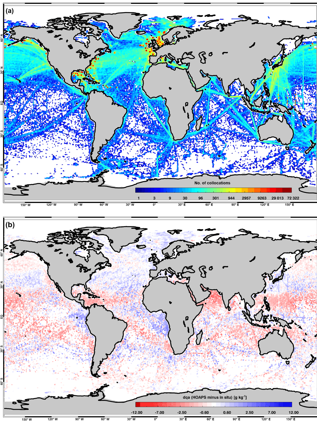
Figure 1. (a) Global map showing the distribution of collocated q_a measurements (HOAPS vs. high-quality in situ) between 2001 and 2008. Overall, more than 13.8 million matchups contribute to this density map. Note that the colour bar is logarithmic. (b) Two-dimensional illustration of the near-surface humidity biases dq_a (HOAPS minus in situ, 2001–2008) shown in Fig. 2. Note that the colour bar is not linear.
