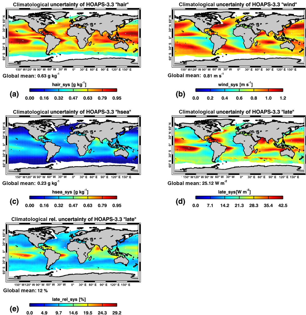
Figure 4. HOAPS 3.3 climatological total uncertainties ( E_{\text{clim}} ) of (a) q_a (“hair”), (b) U (“wind”), (c) q_s (“hsea”), and (d) LHF (“late”). E_{\text{clim}} is defined as the mean root-mean-squared sum of E_{\text{sys}} , E_{\text{retr}}^{\text{ran}} , and E_{\text{smp}} (1988–2012). (e) Climatological mean relative E_{\text{clim}} (LHF) with respect to its natural variability. This variability is defined as the range between the 5th and 95th percentile of instantaneous LHF between 2000 and 2008. The global averages (text strings) were derived by considering a latitudinal cosine dependency. All patterns result from the multi-dimensional bias analyses and subsequent uncertainty propagations described in Sects. 3.2 and 3.4. Note that the colour bar ranges of panels (a) and (c) are identical to allow for direct comparisons.
