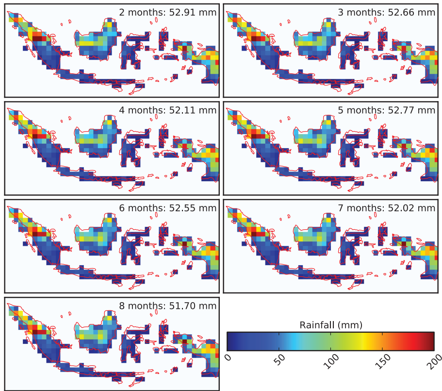
Figure 10. 1997 mean corrected GPCP rainfall rates (per month) during dry season based on using different time frames to convert GPCP to TRMM. The numbers indicate the 1997 mean rainfall for Indonesia during the dry season.
