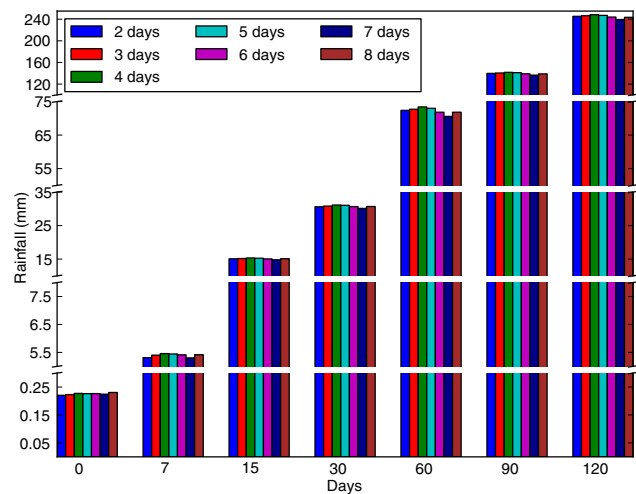
Figure 11. Mean rainfall accumulation before fire in 1997 (based on Fig. 9) in Indonesia with a 0, 7, 15, 30, 60, 90, and 120 days buildup, showing results for all time frames tested to select our correction factor.
