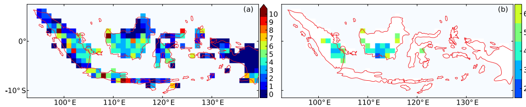
Figure 3. Ratio between MODIS and ATSR (both 22:30 LT overpass) active fire detections over the 2001–2011 overlapping period for (a) all grid cells with active fire detections and (b) only for those grid cells with more than 500 MODIS active fires detected between 2001 and 2011.
