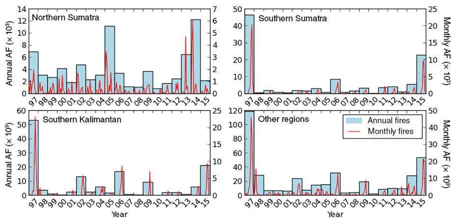
Figure 5. Number of annual (blue bars, left axis) and monthly (red line, right axis) active fire (AF) detections.
