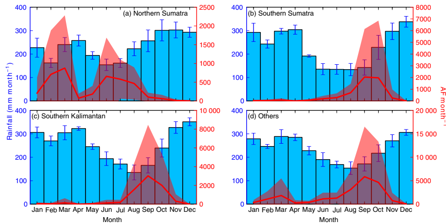
Figure 4. Monthly rainfall with standard deviation (blue) and active fire detections (AF) with standard deviation (red), averaged over 1997–2015.
