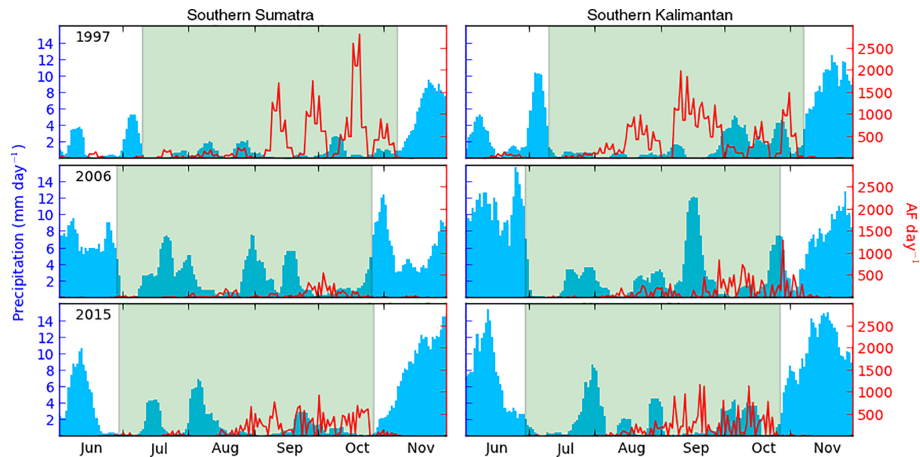
Figure 6. Daily active fire (AF) detections (red) and rainfall (blue) in southern Sumatra and southern Kalimantan during dry seasons of 1997, 2006, and 2015. The green shaded area indicates the dry season defined here as the 120 day period with lowest rainfall.
