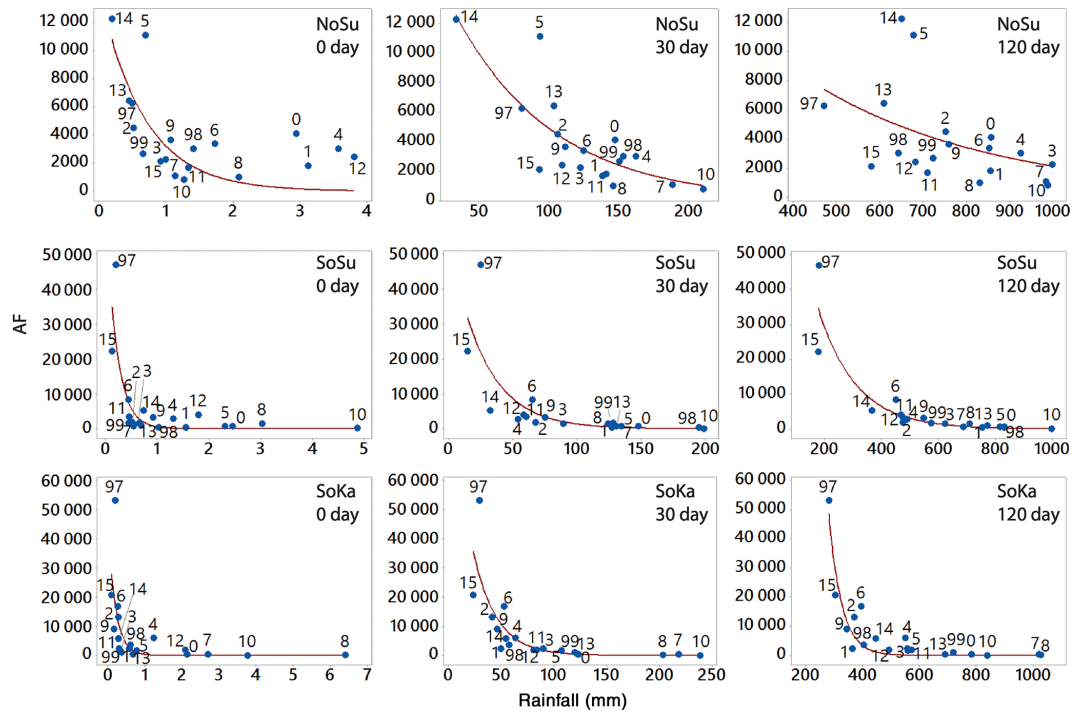
Figure 8. Mean rainfall accumulation before fire (with exponential trend line) for each climatic region with a 0 (left column), 30 (middle column) and 120 days (right column) buildup. The numbers in the graph denote the year (97 is 1997, 0 is 2000, through to 15 is 2015).
