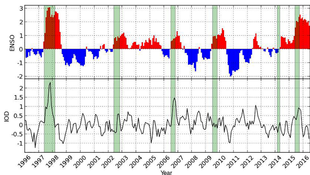
Figure 9. ENSO and IOD with periods of strongest fire activity highlighted in green (more than 5000 AF month -1 ; NOAA, 2016; OOPC, 2016).
