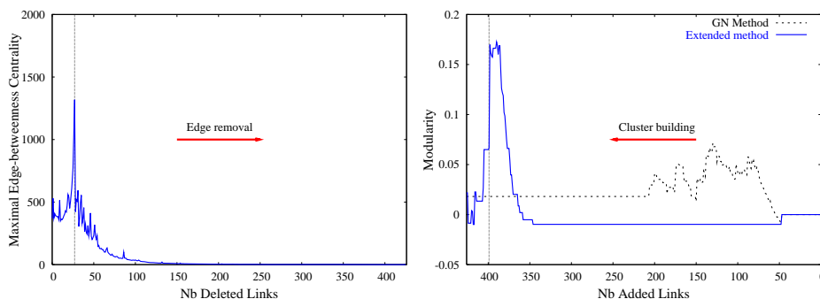
Fig. 3: Left : Maximal edge-betweenness centrality during the edge removal process. Right : Modularity during cluster building with the GN method and the arc-linked cluster detection.
