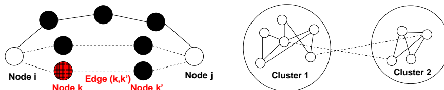
Fig. 1: Left : Node-betweenness and edge-betweenness centralities. Right : Edges between nodes of two clusters have higher edge-betweenness centralities (dashed lines) than edges between nodes of the same cluster (solid lines).
