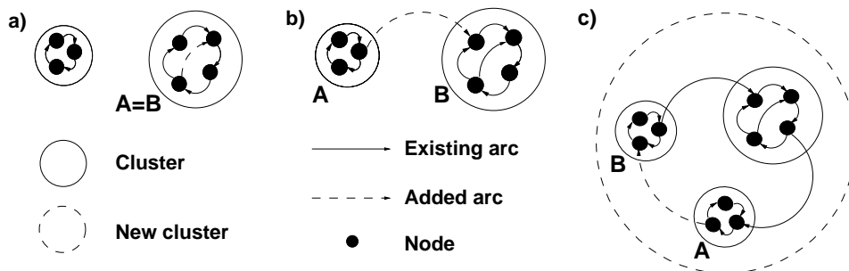
Fig. 2: Description of the construction of arc-linked clusters.
