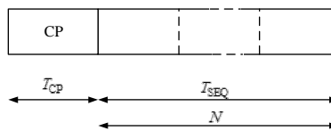
Figure 10.1.6.1-1: Random access symbol group
