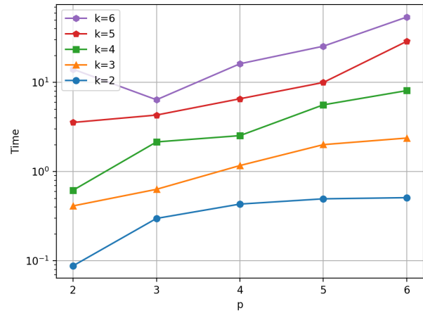
Figure 3: Average computation time in seconds to compute SMMR_{\mathcal{W}}^k(A) with EPI SAT (y-axis) over 20 repetitions varying k and p with an input set of 100 undominated alternatives and \mathcal{W} = \mathcal{U} .
